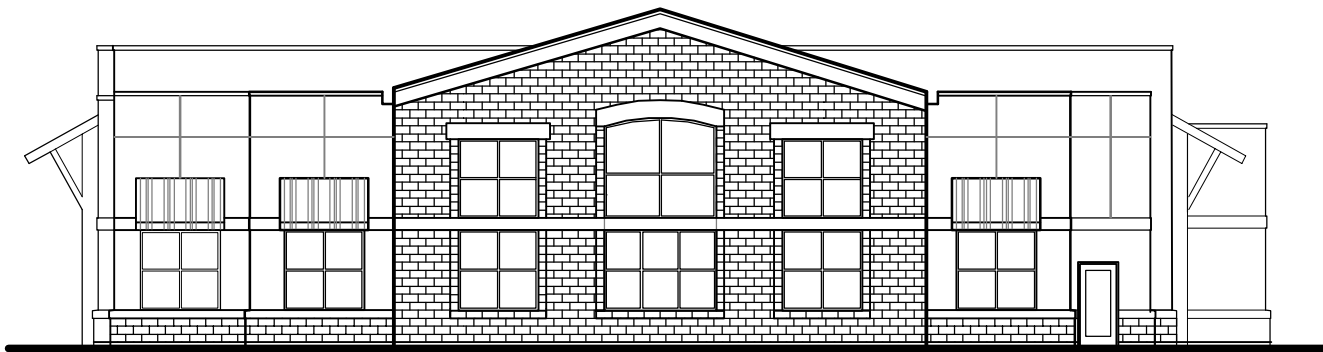
② WEST ELEVATION SCALE: 1/16" = 1'-0"
