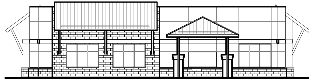
③ EAST ELEVATION SCALE: 1/16" = 1'-0"
